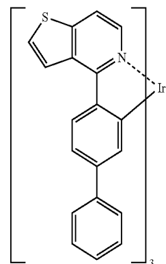
Organic metal compound (VII)
