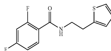
Compound (21)
