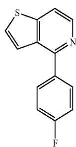
Compound (18)
