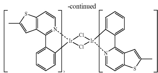
Compound (39)
