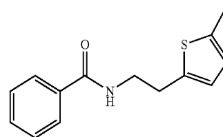
Compound (36)
