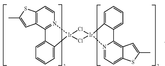
Compound (39)
