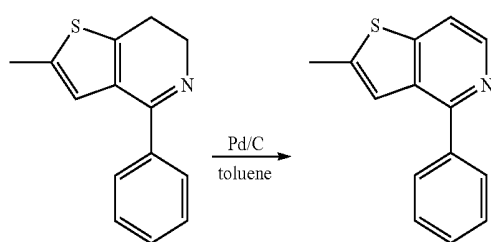
Compound (37)
