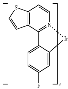
Organic metal compound (IV)
