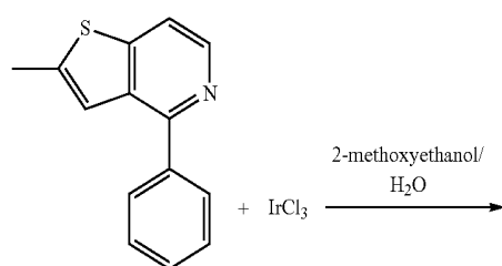
Compound (38)
