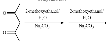
Compound (39)
