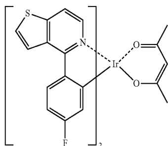
Compound (20)
