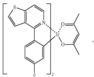
Compound (20)
