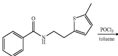
Compound (36)
