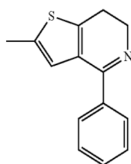
Compound (37)
